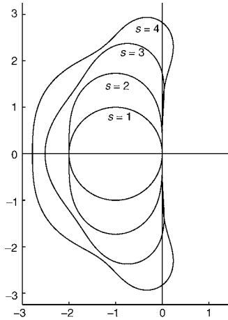
Figure 10.3 Stability regions for Runge–Kutta methods.
